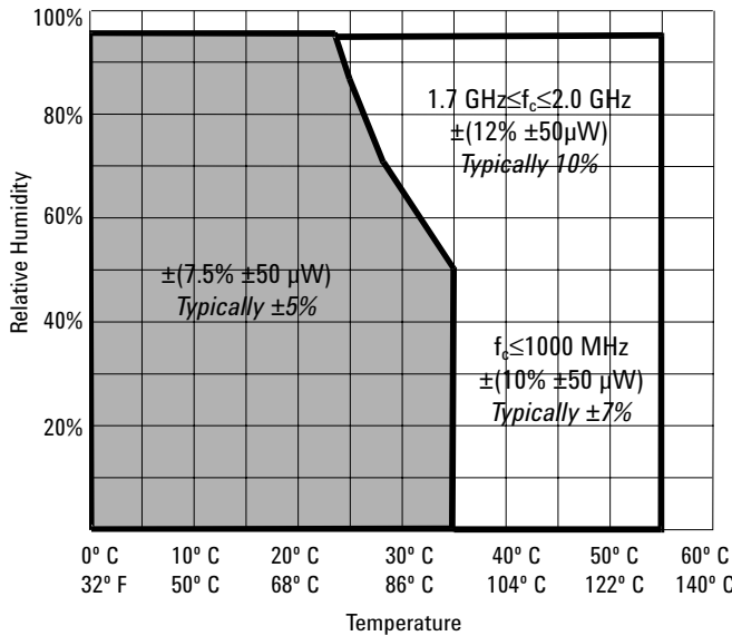
Figure 2. Accuracy
