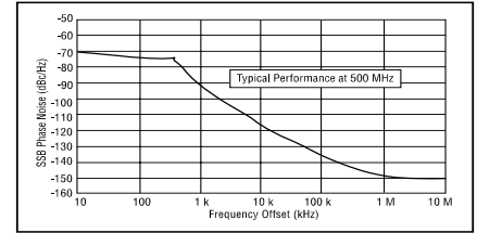
Variation of SSB Phase Noise with Offset
