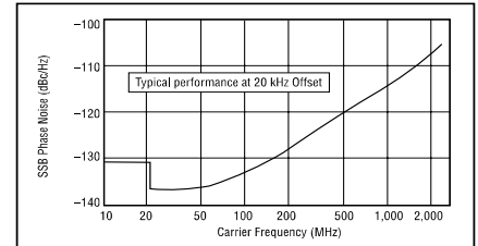
Variation of SSB Phase Noise with Frequency
